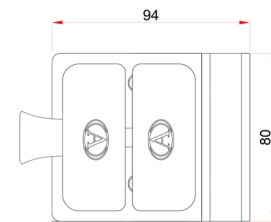
90° Latch Glass to Glass - In
