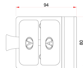
90° Latch Glass to Glass - Out
