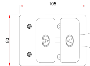
180° Latch Glass to Glass
